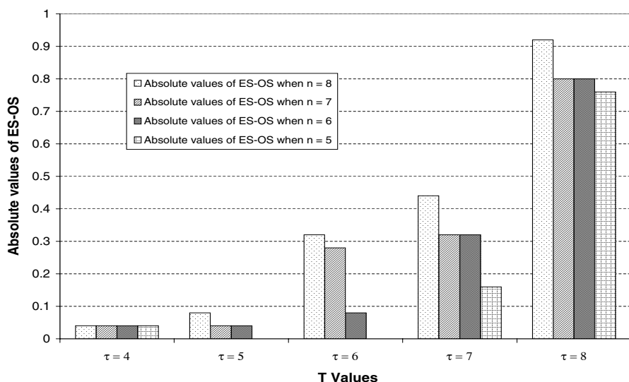
Fig. 15.5. Equilibrium v/s optimal segregation
