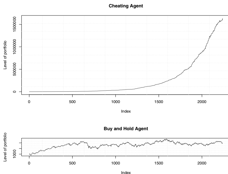
Fig. 5.10. With 0% trans. costs
