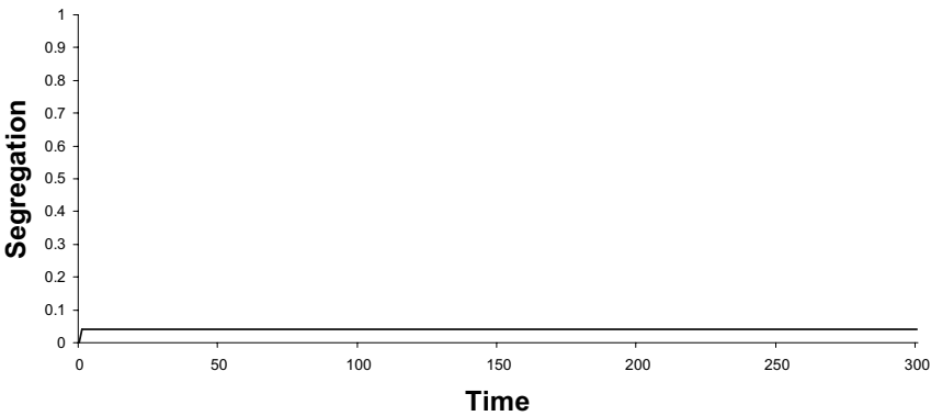
Fig. 15.4. Evolution of segregation
