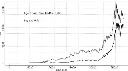
Fig. 5.3. Without trans. costs
