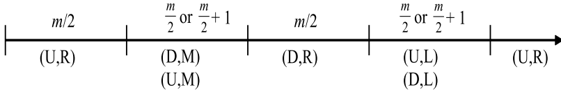
Fig. 19.2. Closed cycle of Markov chain P^m .
