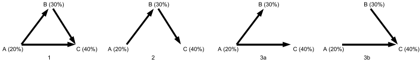
Fig. 14.4. 3-agent network configurations; arrows indicate the lender-borrower pair
