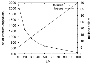
(c) Q: exp. - failures and losses
