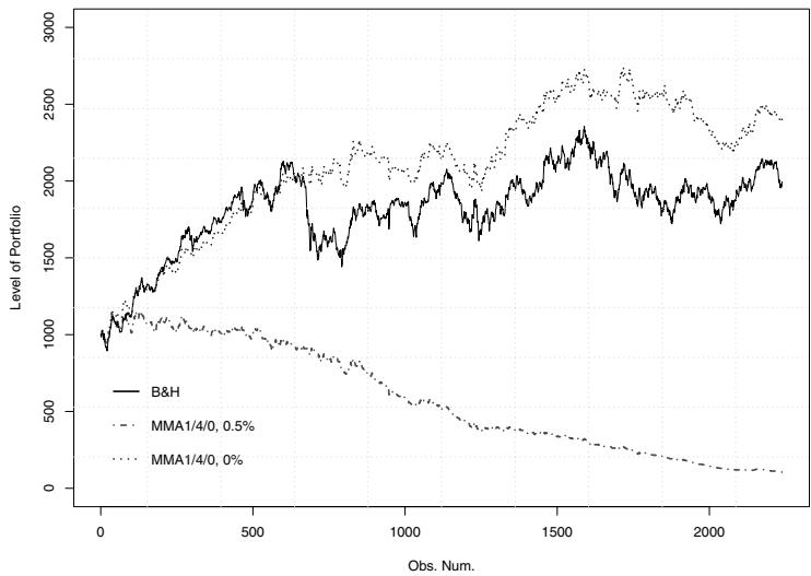
Fig. 5.5. Agents using MMA(1,4) signals
